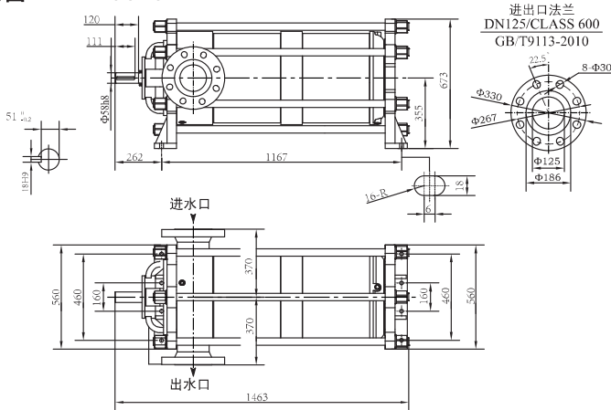
泵体安装图VMHP130-6
