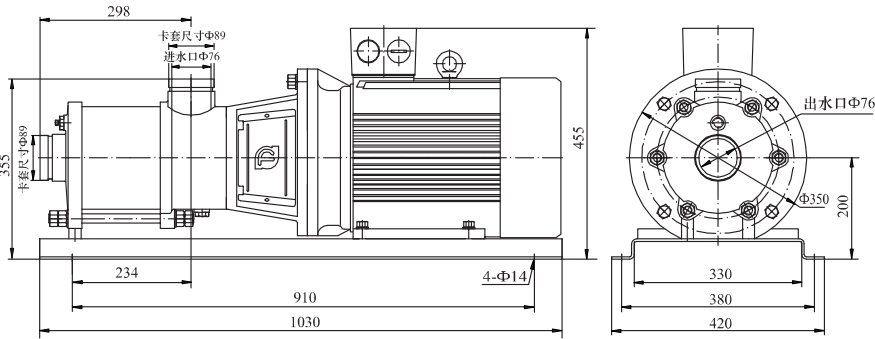
安装图CH62.5-20-1
