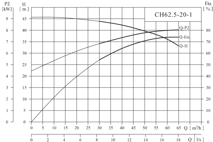
性能表CH62.5-20-1
