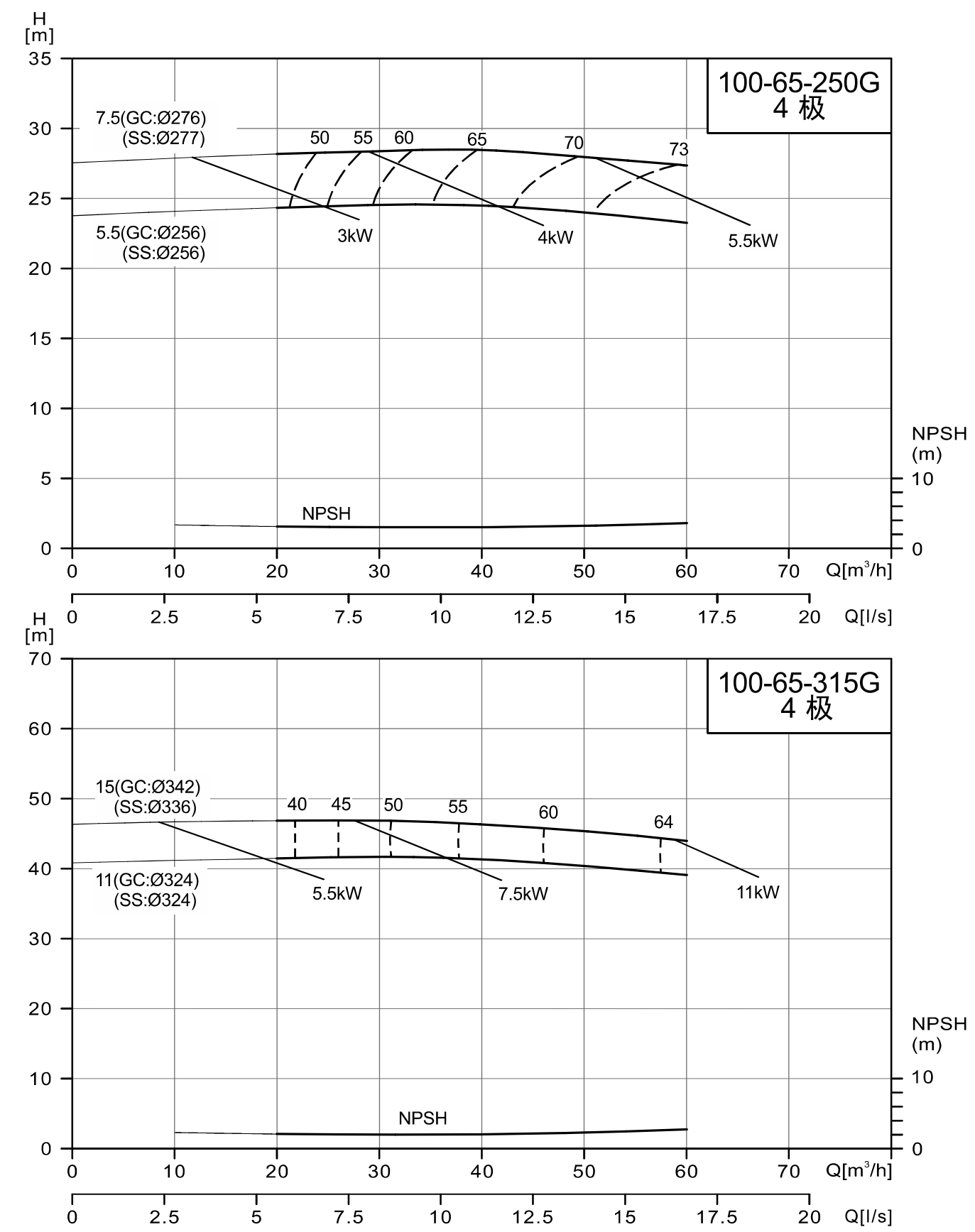
NISO/NIS/NISF100-65-250G/100-65-315G
