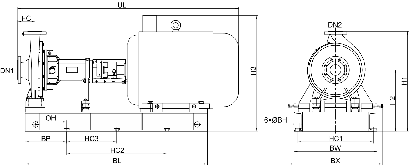
NISO泵组外形尺寸表(槽钢结构)
